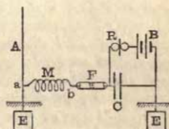
FIG. 19.—SLABY RECEIVER. A, aerial; E, earth plate; F, coherer; M, multiplier; C, condenser; R, relay; B, battery; E, earth plate.
