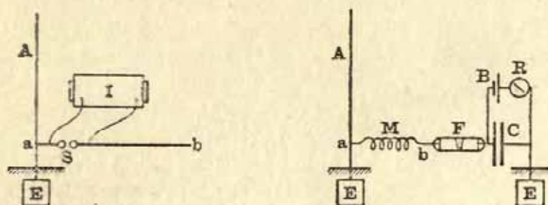
FIG. 24.—SLABY-ARCO SYNTONIC TRANSMITTER AND RECEIVER. I, induction coil; M, multiplier; B, battery; A, aerial; F, filings tube; R, relay; E, earth plate; C, condenser.
