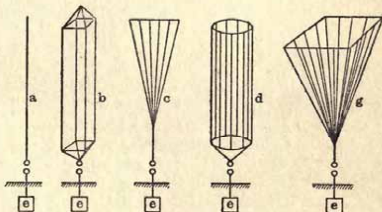
FIG. 8.—VARIOUS FORMS OF AERIAL RADIATOR.
