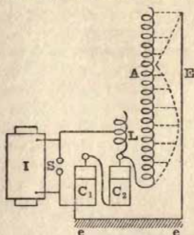
FIG. 11.—HARMONIC OSCILLATIONS IN LONG SOLENOID SHOWN WITH SEIST'S APPARATUS.
