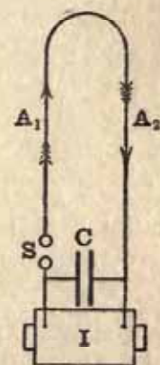
FIG. 12.—NON-RADIATIVE CLOSED LOOP AERIAL.
