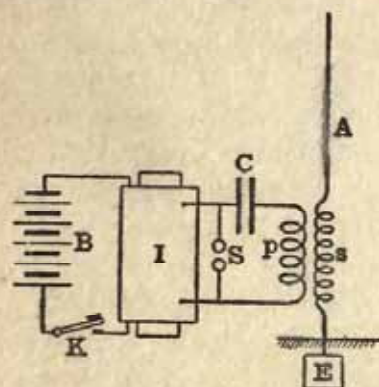
FIG. 9.—MARCONI-BRAUN SYSTEM OF INDUCING ELECTROMOTIVE FORCE IN AN AERIAL, A, B, battery; K, key; I, induction coil; S, spark gap; C, Leyden jar; E, earth plate; P, oscillation transformer.
