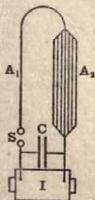
FIG. 13.—SLABY'S LOOP RADIATOR.
