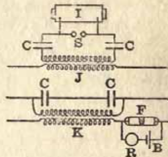
FIG. 21.—BRAUN'S NON-EARTHED RECEIVER. I, induction coil; CC, condensers; S, spark gap; J, transmitting jig; K, receiving jig; F, filings tube; R, relay; B, battery.
