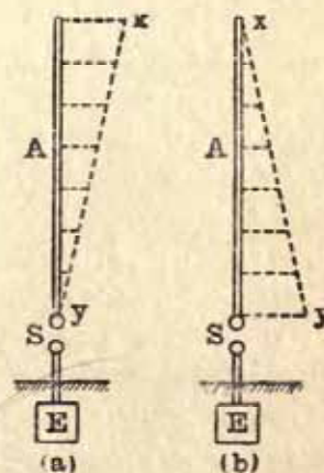
FIG. 6.—(a) DISTRIBUTION OF ELECTRIC PRESSURE IN A MARCONI AERIAL, A, (b) DISTRIBUTION OF ELECTRIC CURRENT IN A MARCONI AERIAL, AS SHOWN BY THE ORDINATES OF THE DOTTED LINE xy .
