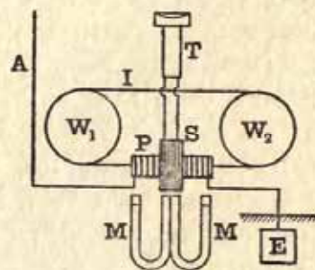
FIG. 18.—MARCONI MAGNETIC RECEIVER. W_1W_2 , wheels; I, iron wire band; P, primary coil; S, secondary coil; T, telephone; A, aerial; E, earthplate.
